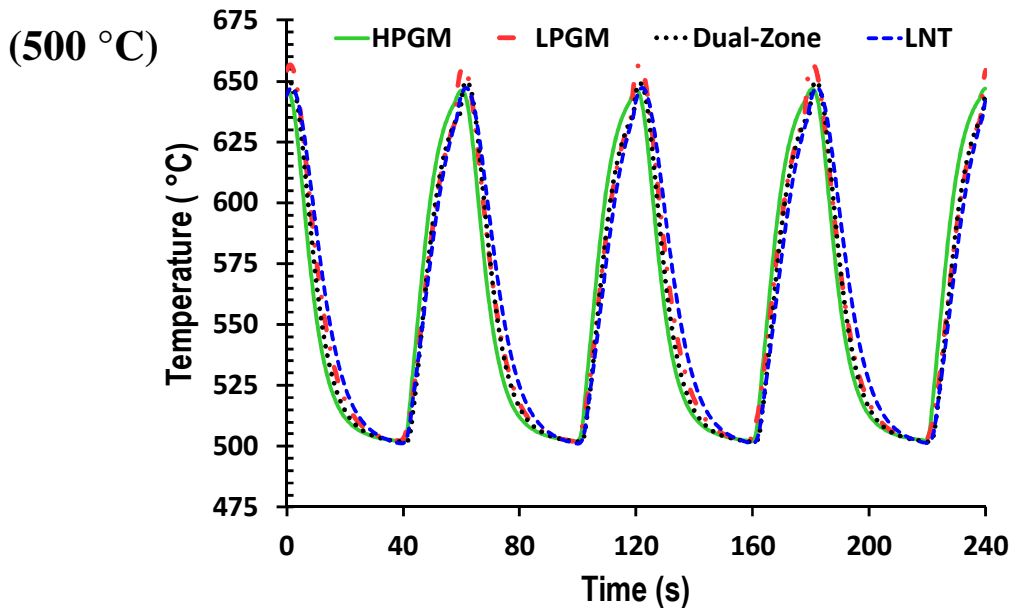
Figure 60. Typical temperature exotherms observed the HPGM, LPGM, Dual-Zone and LNT catalysts during cycling at 250 and 500 °C, respectively. (Rich period AFR = 14.2).
