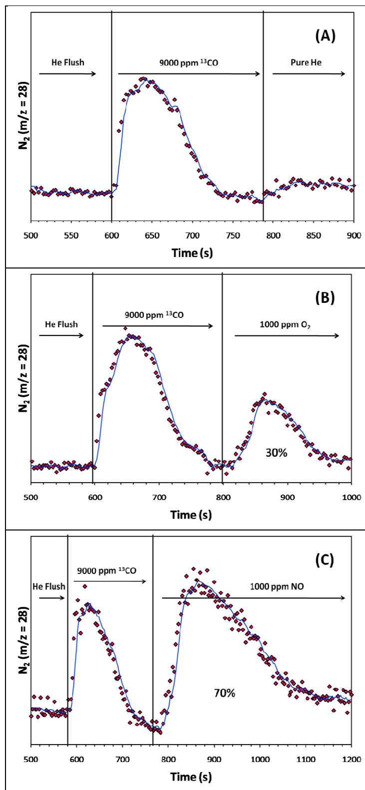
Figure 37. N_2 profiles ( m/z = 28 ) obtained during the reaction of stored NO_x with ^{13}CO and the subsequent reaction of residual NCO species with (A) He, (B) 1000 ppm O_2/He or (C) 1000 ppm NO/He on Rh/Ba/Al_2O_3 at 350 °C.
