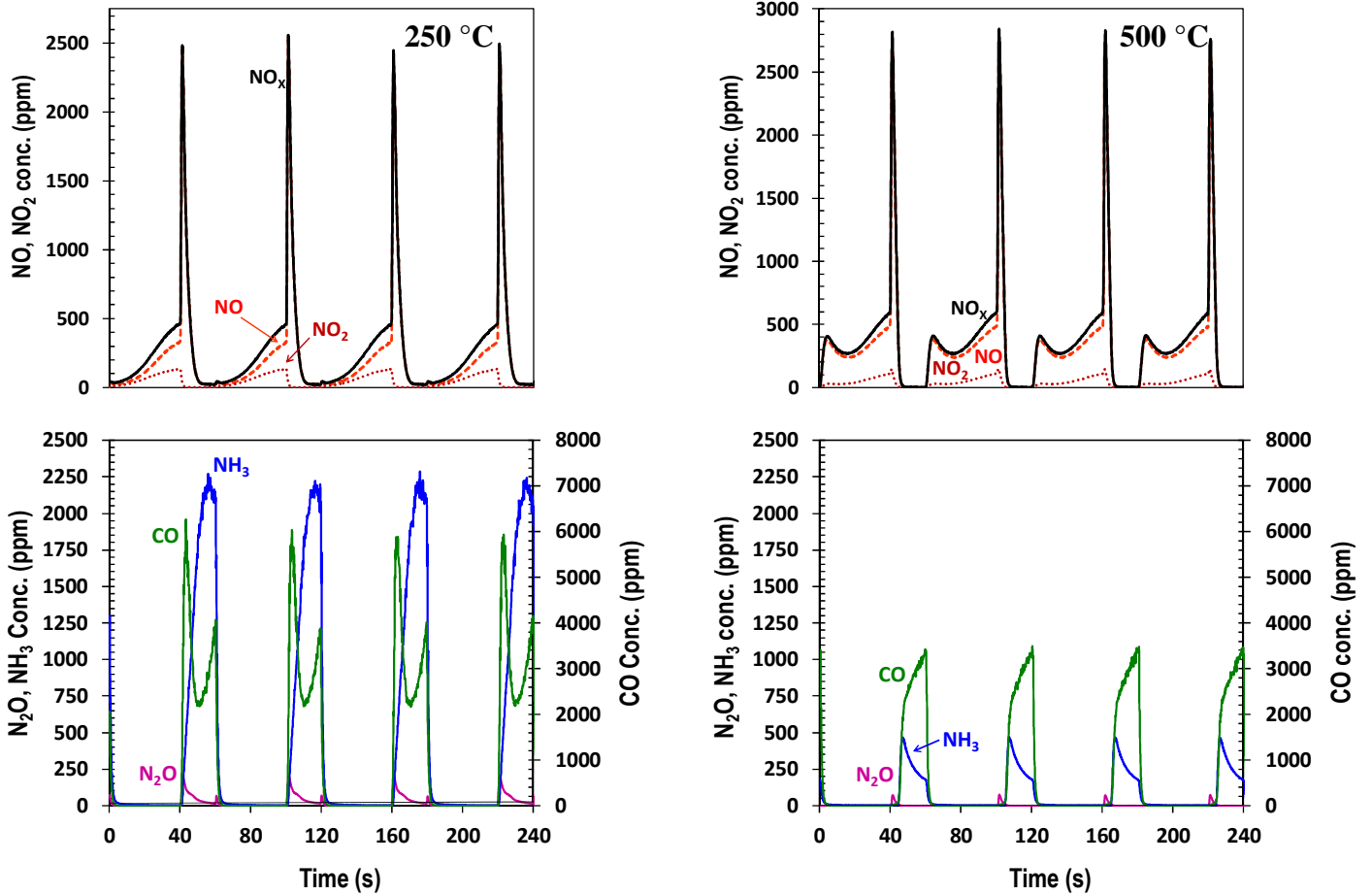
Figure 59. Lean/rich cycling over LNT as TWC at 250 and 500 °C, respectively. (Same conditions as Fig. 56)
