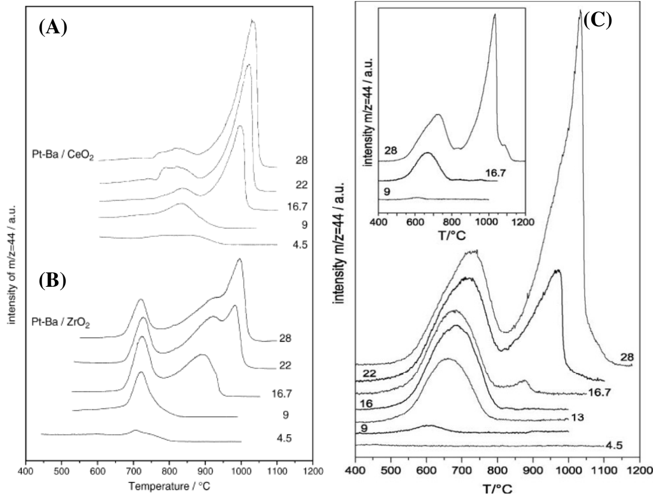
Figure 15. CO 2 evolution profiles of BaCO 3 decomposition formed during calcination at 500 °C of the Ba(Ac) 2 precursor for varying loadings of Ba on different supports where (A) Pt-Ba/CeO 2 , (B) Pt-Ba/ZrO 2 and (C) Pt-Ba/Al 2 O 3 . Pt-Ba/SiO 2 not shown, Piacentini et al. [161,228].
