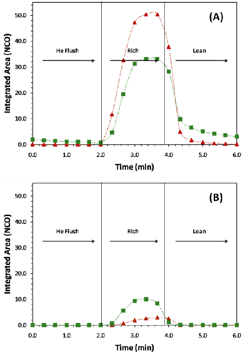
Figure 34. Comparison between the amounts of NCO species formed on (▲) Pt/Ba/Al 2 O 3 and (■) Rh/Ba/Al 2 O 3 at 350 °C in the absence of H 2 O (Lean: 1000 ppm NO/5% O 2 /He; Rich: pane (A) 9000 ppm CO/He; pane (B) 1000 ppm C 3 H 6 /He).
