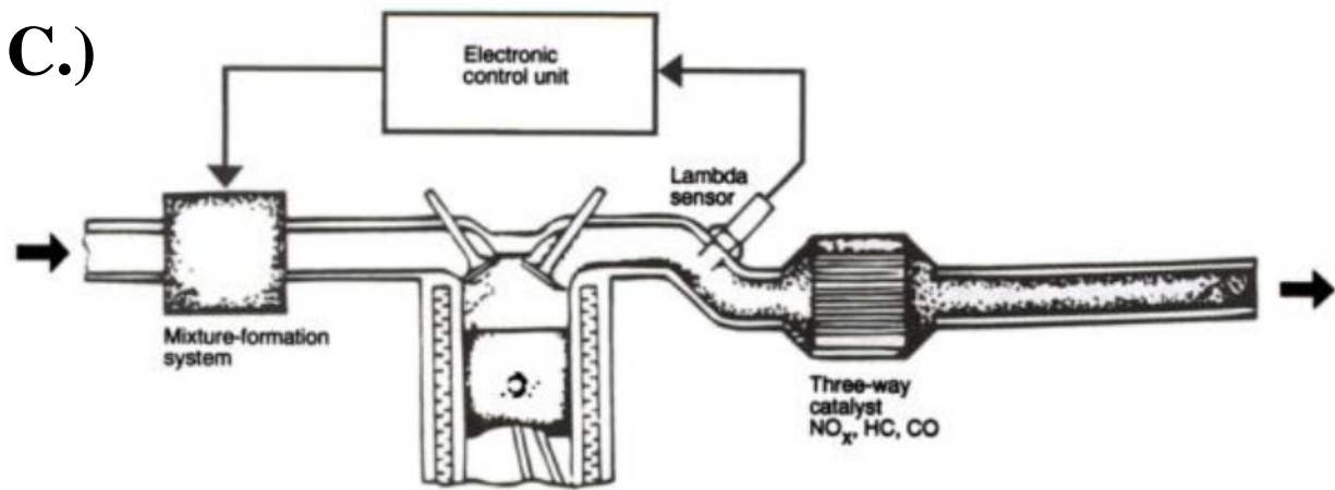
SINGLE BED THREE-WAY CATALYTIC CONVERTER
