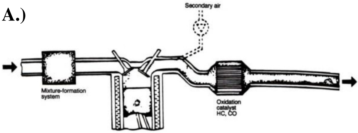
SINGLE BED OXIDATION CATALYTIC CONVERTER
