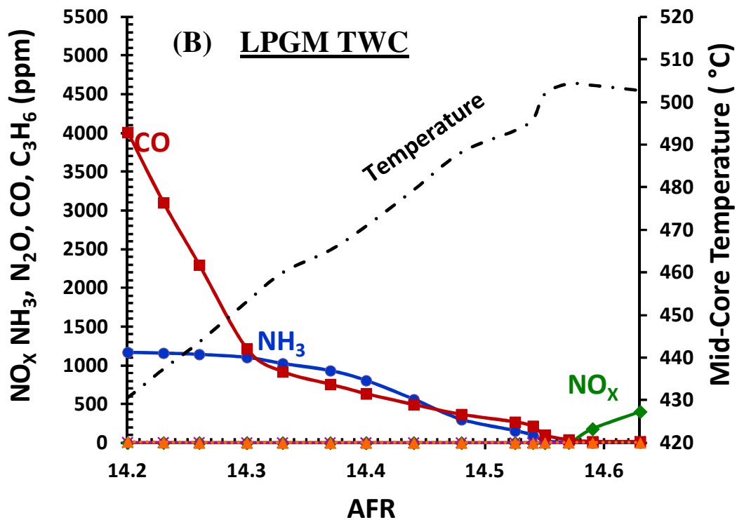
Figure 52. Effluent gas concentrations for (◆) NO x , (●) NH 3 (×) N 2 O, (■) CO and (▲) C 3 H 6 over (A) HPGM, Pd-only TWC and (B) LPGM, Pd/Rh TWC, respectively. (S.V. 75,000 hr -1 , Inlet Temp. = 250 °C, Reaction conditions shown in Table. 12).
