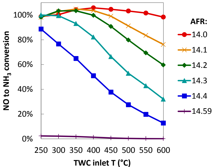
Figure 55. Quantified \text{NH}_3 yield over the HPGM, Pd-only TWC as a function of the AFR and temperature.
