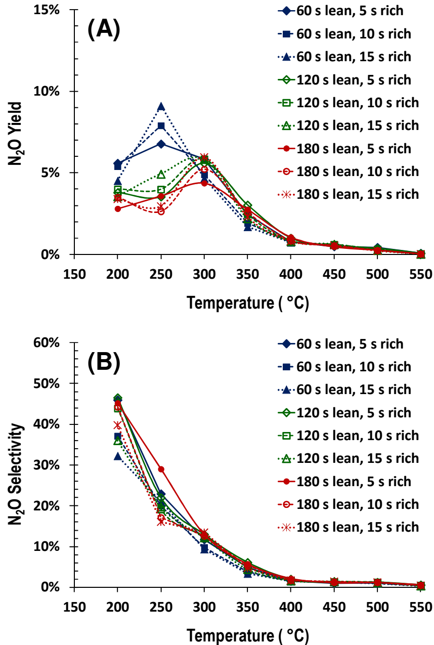
Figure 49. Cycle averaged N_2O yield (A) and selectivity (B) obtained for the LNT catalyst as functions of temperature and lean/rich cycle timing.
