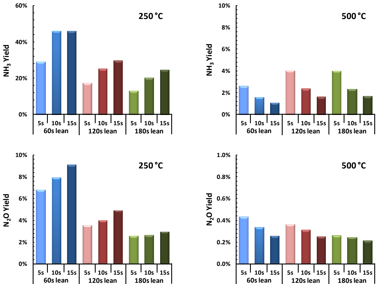
Figure 50. Cycle averaged \text{NH}_3 and \text{N}_2\text{O} yields obtained for the LNT catalyst for different lean/rich cycle timing protocols at 250 and 500 °C.
