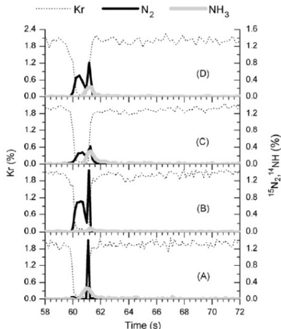
Figure A28. Evolution of reaction products during a rich event ( \text{CO} + \text{H}_2 + \text{H}_2\text{O} + \text{CO}_2 ) at 350^\circ\text{C} on a series of NSR catalysts formulated from commonly used precious metals including: (A) 0.5% Pt, (B) 1.6% Pt, (C) 1.1% Rh and (D) 0.5% Pt-0.8% Rh supported on 17%Ba/Al 2 O 3 (w/w), Breen et al. [16].
