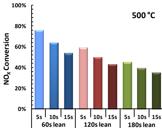
Figure 44. Cycle averaged NO x conversions obtained for the LNT catalyst for different lean/rich cycle timing protocols at 250 and 500 °C.
