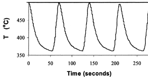
Figure A19. Temperature profile of the catalyst bed during 60 s lean, 10 s rich periods over 2.2\% \text{Pt}/16.3\% \text{BaO}/\text{Al}_2\text{O}_3 (w/w), where lean: 500 ppm \text{NO} , 5% \text{O}_2 , 1000 ppm \text{C}_3\text{H}_6 and rich: 500 ppm \text{NO} , 5% \text{O}_2 , 1.4% \text{C}_3\text{H}_6 . Reprinted from Kabin et al., 2004 [18].
