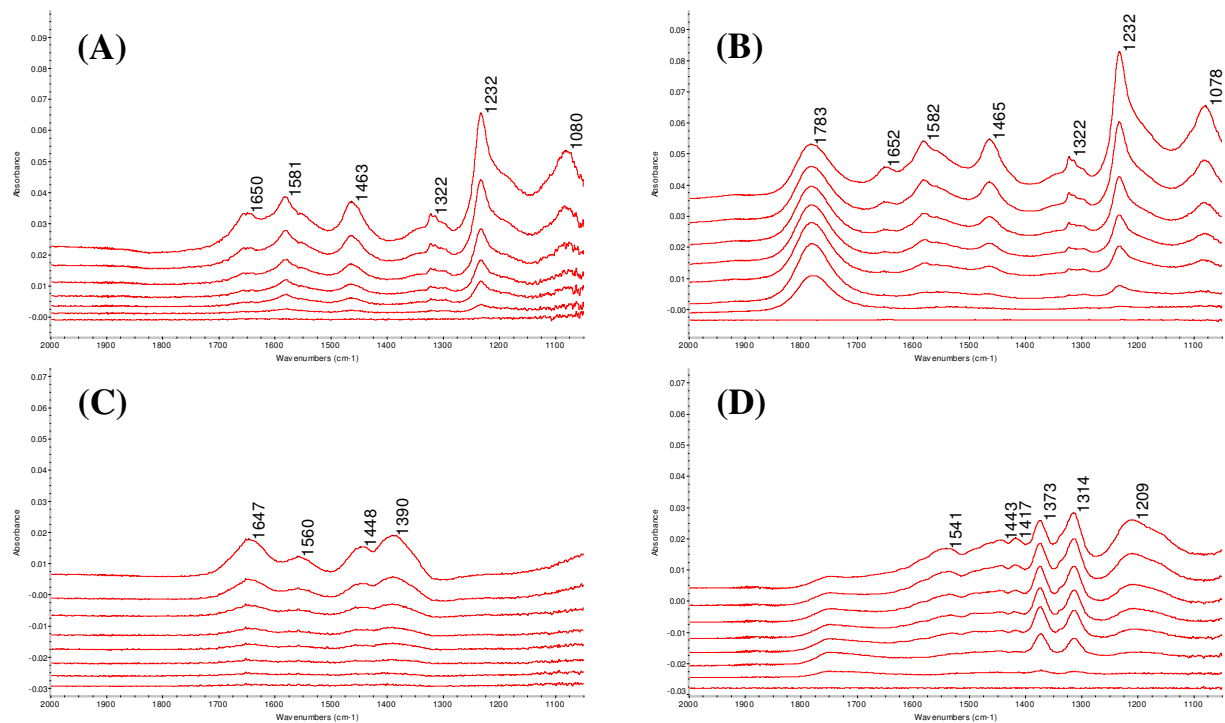
Figure A1. Adsorption of 1000 ppm NO in He at RT on (A) \text{Al}_2\text{O}_3 , (B) \text{Pt}/\text{Al}_2\text{O}_3 , (C) \text{Ba}/\text{Al}_2\text{O}_3 , (D) \text{Pt}/\text{Ba}/\text{Al}_2\text{O}_3 . Spectra shown after 0, 0.5, 1, 2, 3, 5, 10 & 20 min., respectively.
