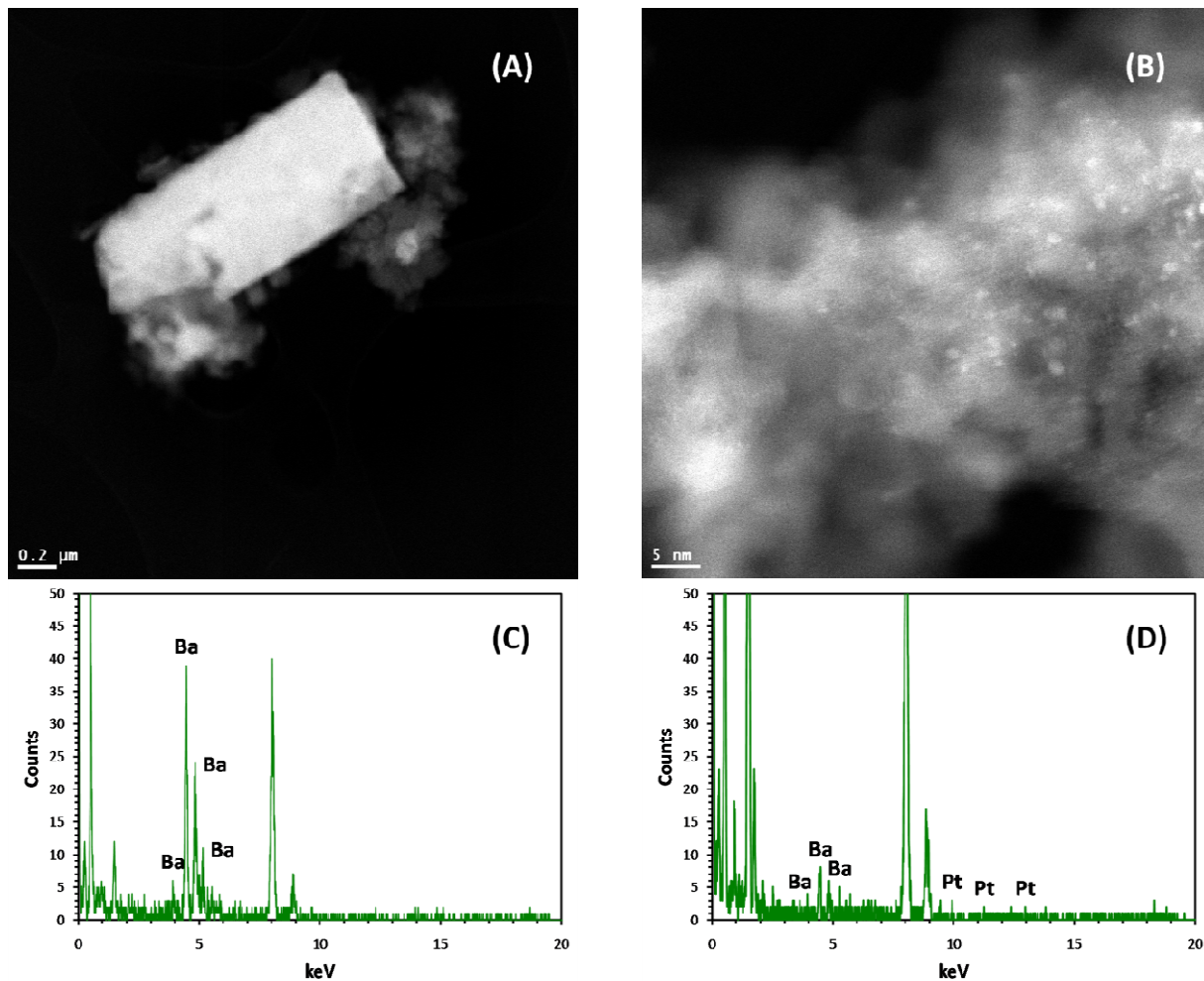
Figure 26. STEM images and corresponding EDX analyses of two different regions of the Pt/Ba/Al 2 O 3 catalyst used in this investigation.
