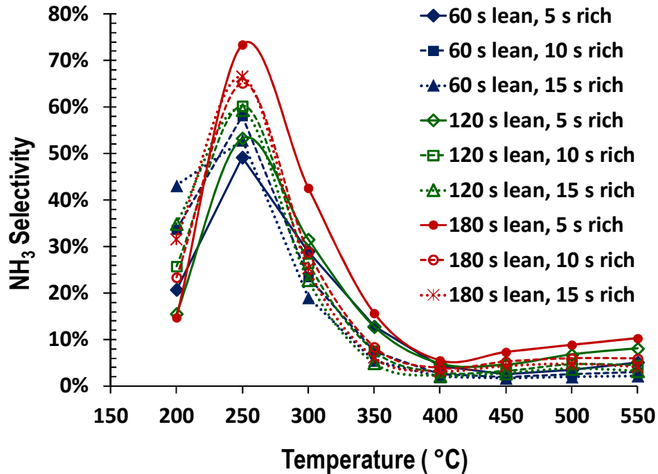
Figure 48. Cycle averaged \text{NH}_3 selectivity obtained for the LNT catalyst as a function of temperature and lean/rich cycle timing.
